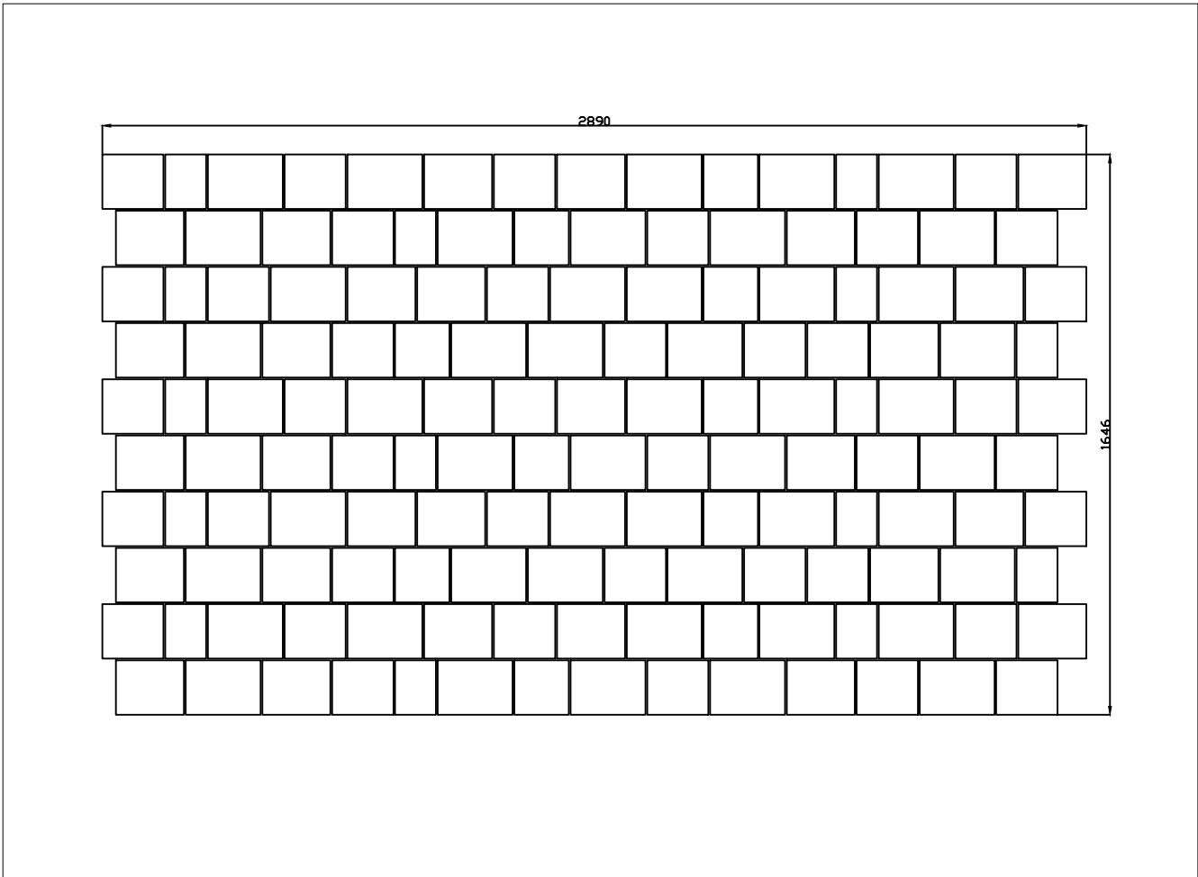
Random course laying pattern (Joint width 3 - 5mm)
