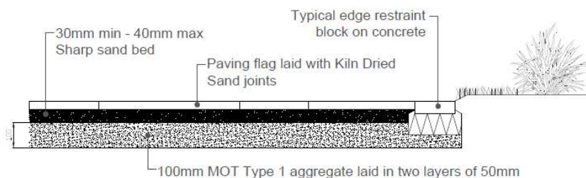
2 Typical section through a patio constructed in accordance with Marshalls Register Installation Procedures D01 Scale 1:20 @ A3
