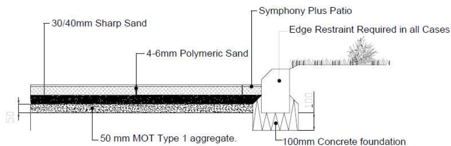
15 Typical section through a patio constructed in accordance with Marshalls Register Installation Procedures D02 Scale 1:20 @ A3
