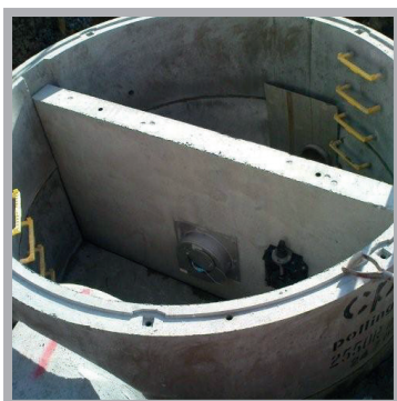
2550mm wide wall chamber installed complete with Hydro-Brake® and penstock on weir wall.
