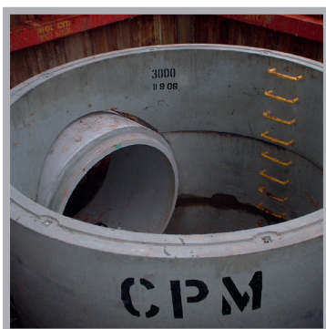
3000mm wide wall sectional chamber, 1800mm inlet and 1050mm outlet, pre-fitted Hydro-Brake® and penstock.
