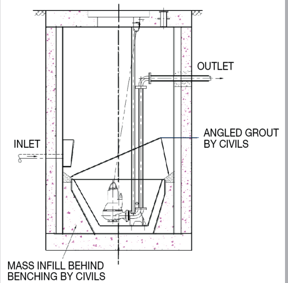
2100mm Pump Chamber
