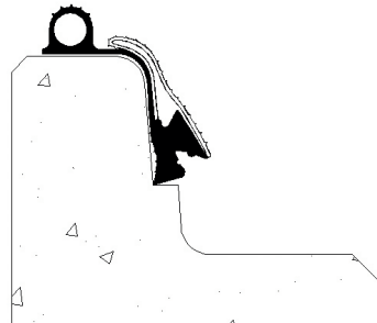
Forsheda - F171 Seal
