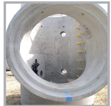
1500mm integrated flow control for attenuation tank
