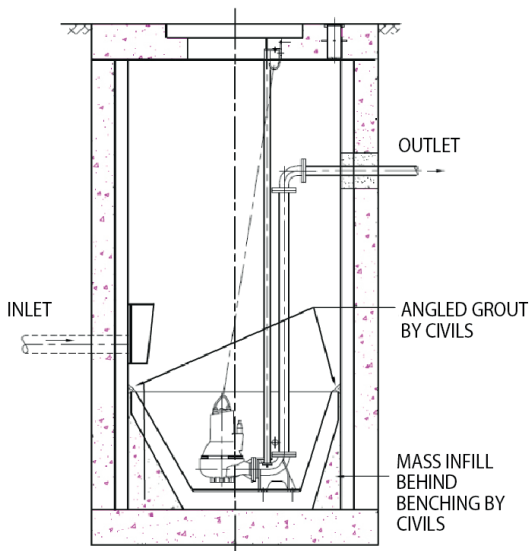
1800mm Plus Pump Chamber
