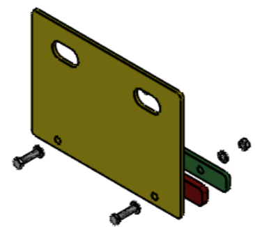
LIFTING KIT ASSY (EXPLODED VIEW) SCALE 1 : 10
