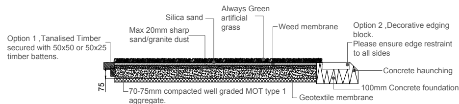
9 Typical section through an Always Green Lawn installed in accordance with Marshalls Register Installation Procedures D03 Scale 1:20 @ A3
