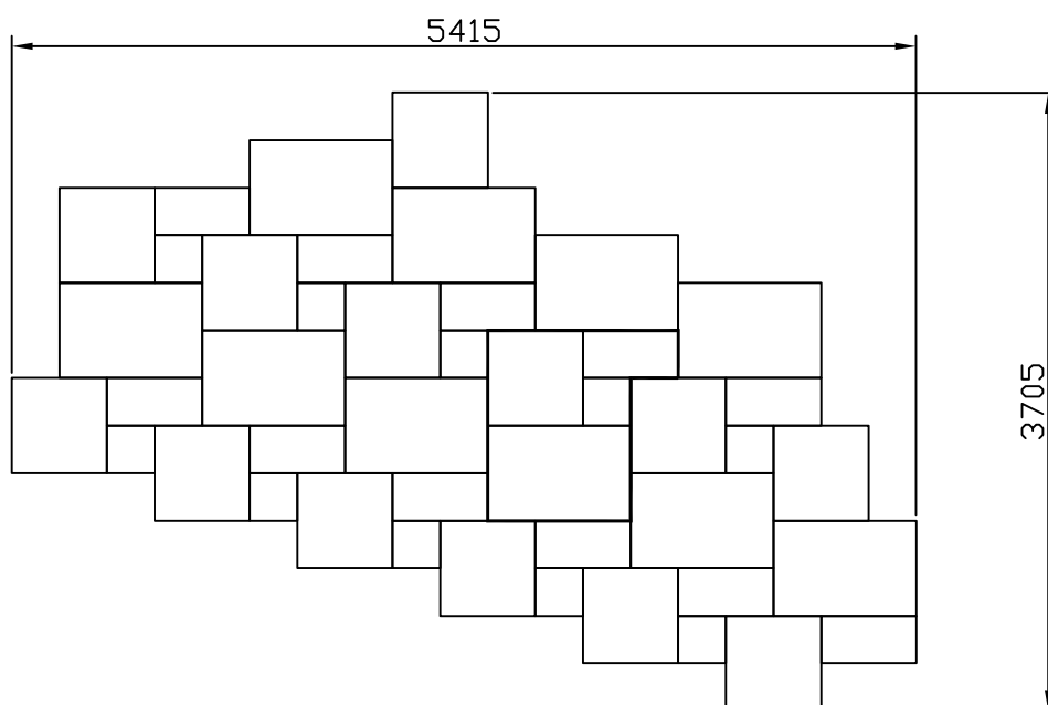
Option 2 - Repeatable Pattern (8-15mm nominal joint required)
