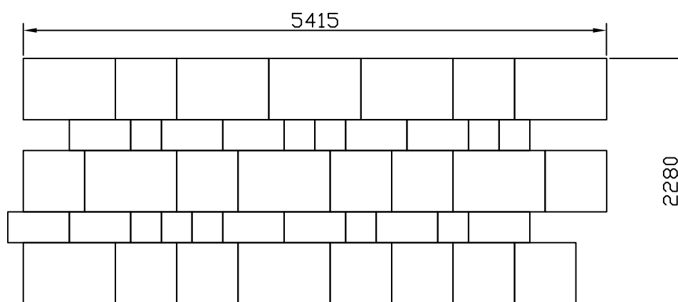
Option 1 - Random Stretcher Course Pattern (8-15mm nominal joint required)
