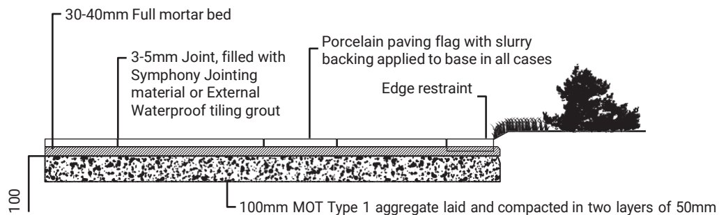
3 Typical section through a patio constructed in accordance with Marshalls Register Installation ProceduresD01 Scale 1:20 @A3
