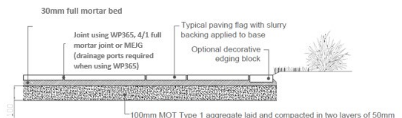
1 Typical section through a patio constructed in accordance with Marshall's Register Installation Procedures D01 Scale 1:20 @ A3
