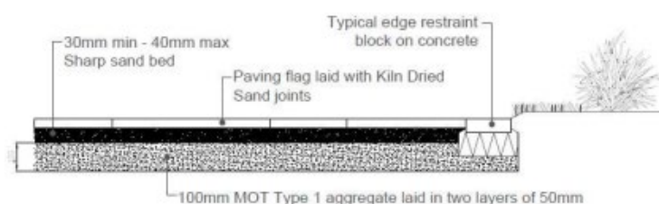
2 Typical section through a patio constructed in accordance with Marshalls Register Installation Procedures D01 Scale 1:20 @ A3
